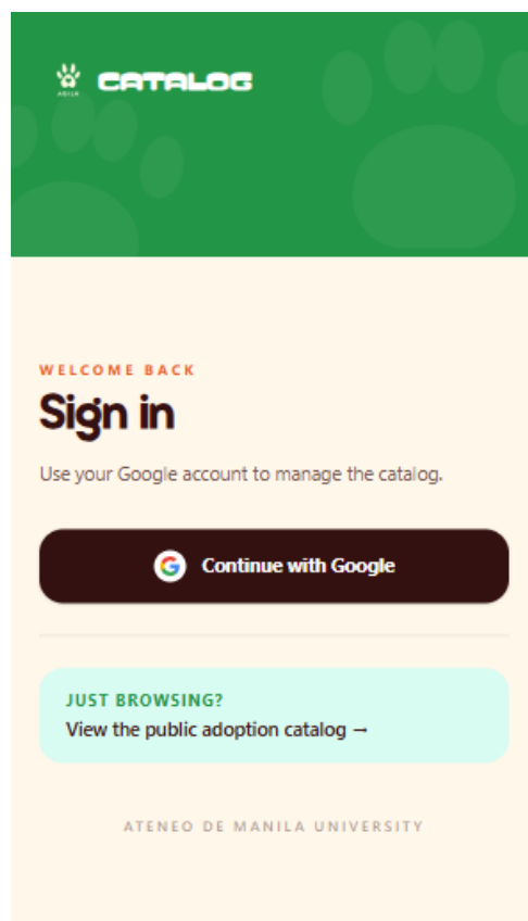
Figure 1: Sign-In Screen
