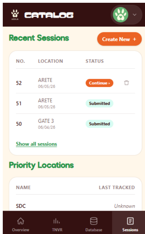
Figure 2: Sessions Tab
