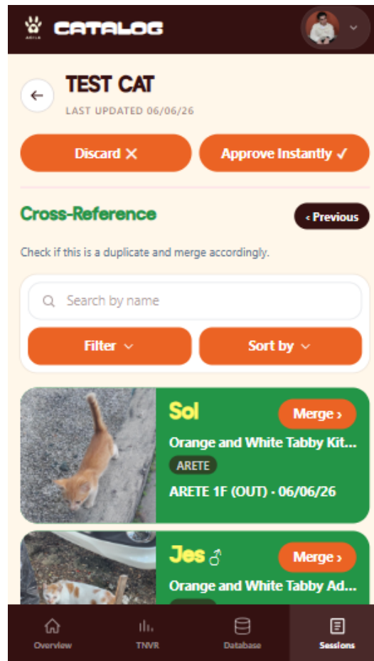
Figure 8: Cross-Reference Screen
