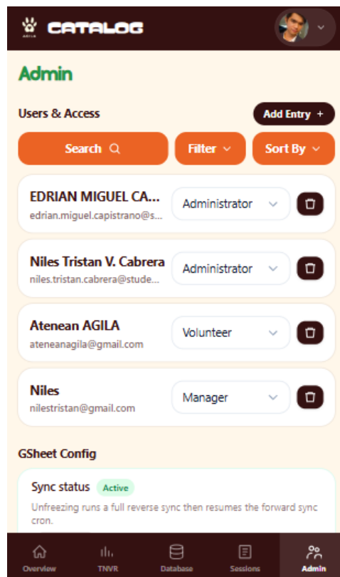
Figure 10: Admin Tab
